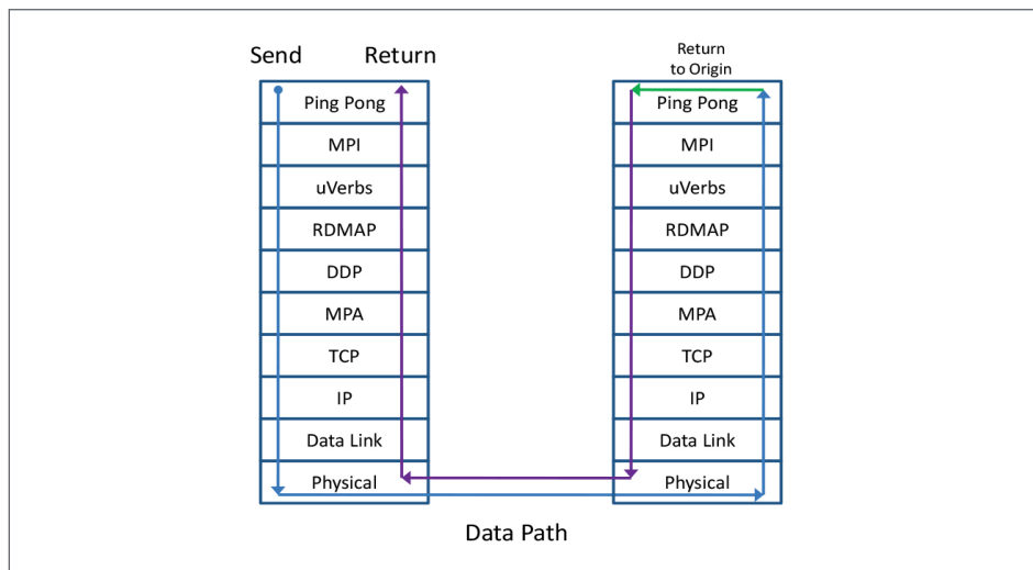
Figure 2. Ping Pong - Data Path
