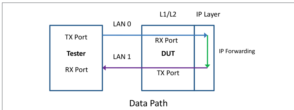
Figure 4. RFC2544 Latency Testing via IP Forwarding
