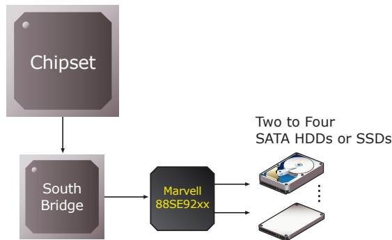
Fig 2. RAID-On-Motherboard Application
