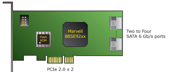
Fig 3. SATA RAID HBA Application
