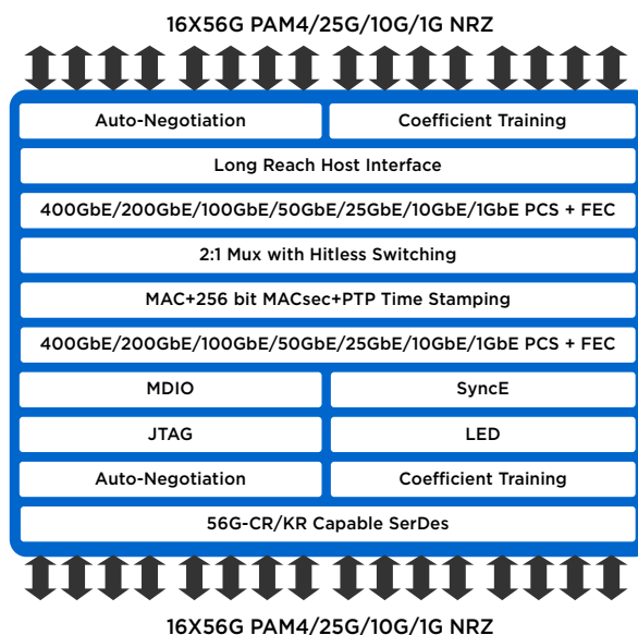
Marvell 88X7121P Block Diagram
