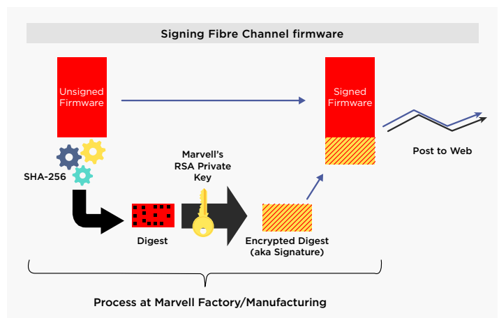
Figure 2. Marvell signing trusted firmware using RSA private key
