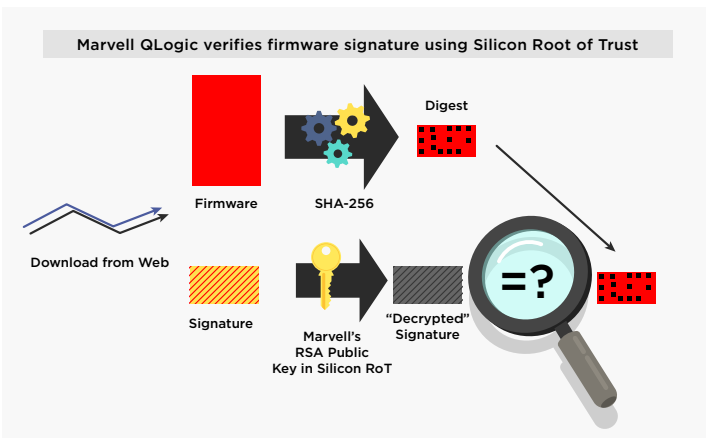
Figure 1. Marvell QLogic 2770 Series firmware verification using RSA public key
